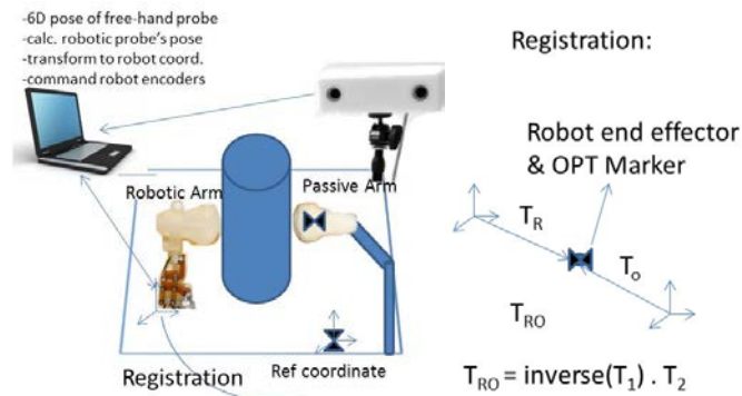
Figure 2. Project Schematics
