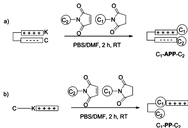
Figure 3. One-step synthesis of the photoacoustic probes. (a) Two probes were synthesized with the ACP platform, Ceee[Ahx]PLGLAGrrrrK: one where C_1 = BHQ3 and C_2 = Alexa750 (B-APP-A), and the other where C_1 = QXL680 and C_2 = Hilyte750 (Q-APP-H). Two other probes, B-PP-A and Q-PP-H, had the same combination of the dyes but a different peptide platform, CGVRPLKrrrr (b). The small letters signify D-amino acids.
