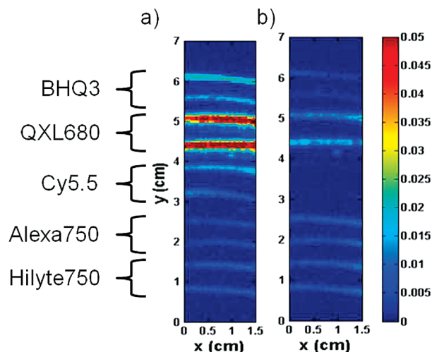
Figure 2. Photoacoustic imaging of the chromophores. Polyethylene capillaries were filled with 10 \mu\text{M} solution of various dyes and imaged at 675 (a) and 750 nm (b). The samples were done in duplicate. The first two dyes are quenchers, BHQ3 ( \lambda_{\text{abs}} = 672 nm) and QXL680 ( \lambda_{\text{abs}} = 679 nm), while the other three are fluorophores, Cy5.5 ( \lambda_{\text{abs/em}} = 675/694 nm), Alexa750 ( \lambda_{\text{abs/em}} = 749/775 nm), and Hilyte750 ( \lambda_{\text{abs/em}} = 754/778 nm). The color bar on the right represents relative photoacoustic signal and corresponds to both (a) and (b). x and y represent the vertical and horizontal lengths of the area of the agar that was scanned.
