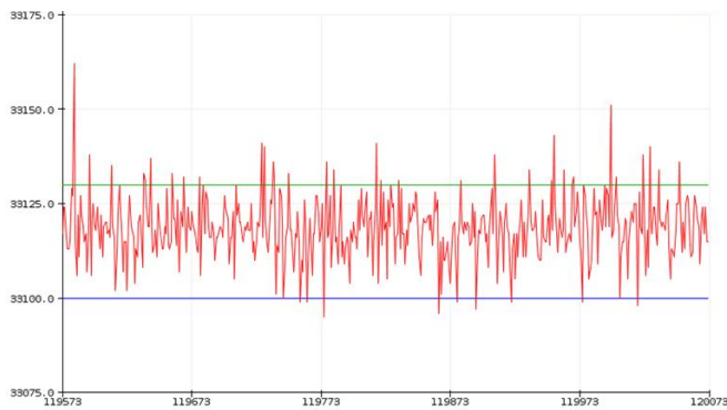
Figure 10: Digitized 16-bit voltage readings in red of third trial at last 500 samples; lines used to control upper and lower axis limits for voltage are in green and blue
