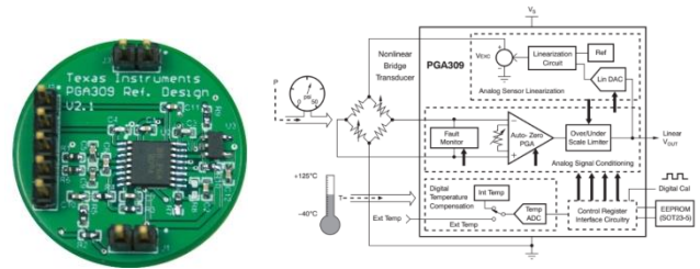
Figure 4: Physical view and simplified block diagram of PGA309 package
