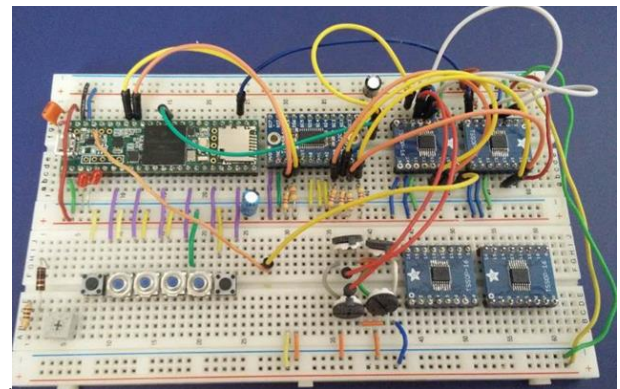
Figure 9: Breadboard mockup prototype of data acquisition board
