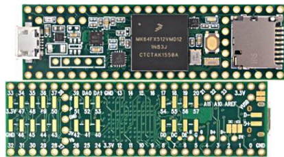
Figure 3: Front and back view of Teensy 3.5 USB board
