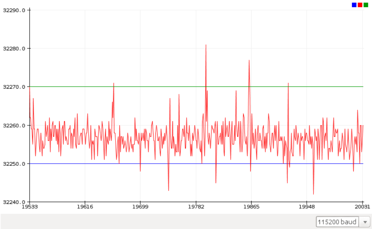
Figure I5: 32-sample averaging; high sampling speed; high conversion speed
