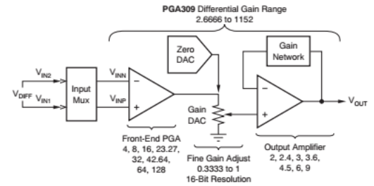
Figure 5: Three-stage amplifier subsystem schematic and gain function
