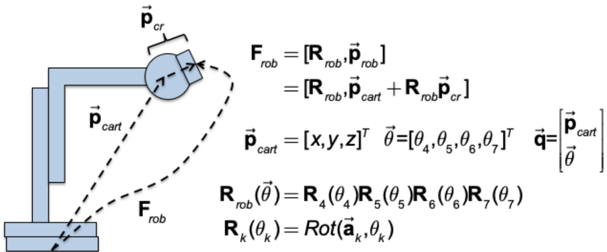
Fig. 1: Robot Kinematics
