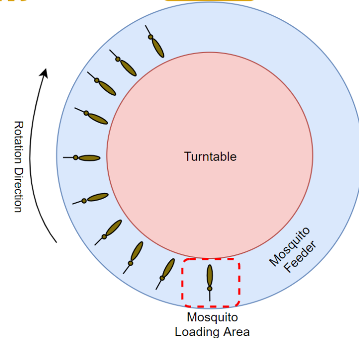
Figure 3. System Diagram
