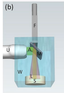
Figure 1. Example showing how an acoustic mirror works. [1] (M is the acoustic mirror, U is the ultrasound probe, A is the ultrasound wave emitted by the probe, and W is the water. Other components are not important for Patch Ultrasound)
