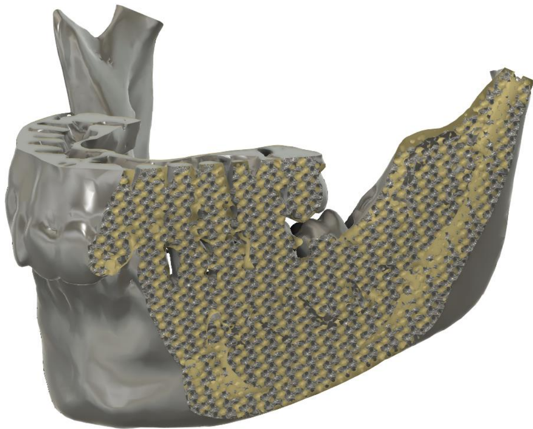
Section View
