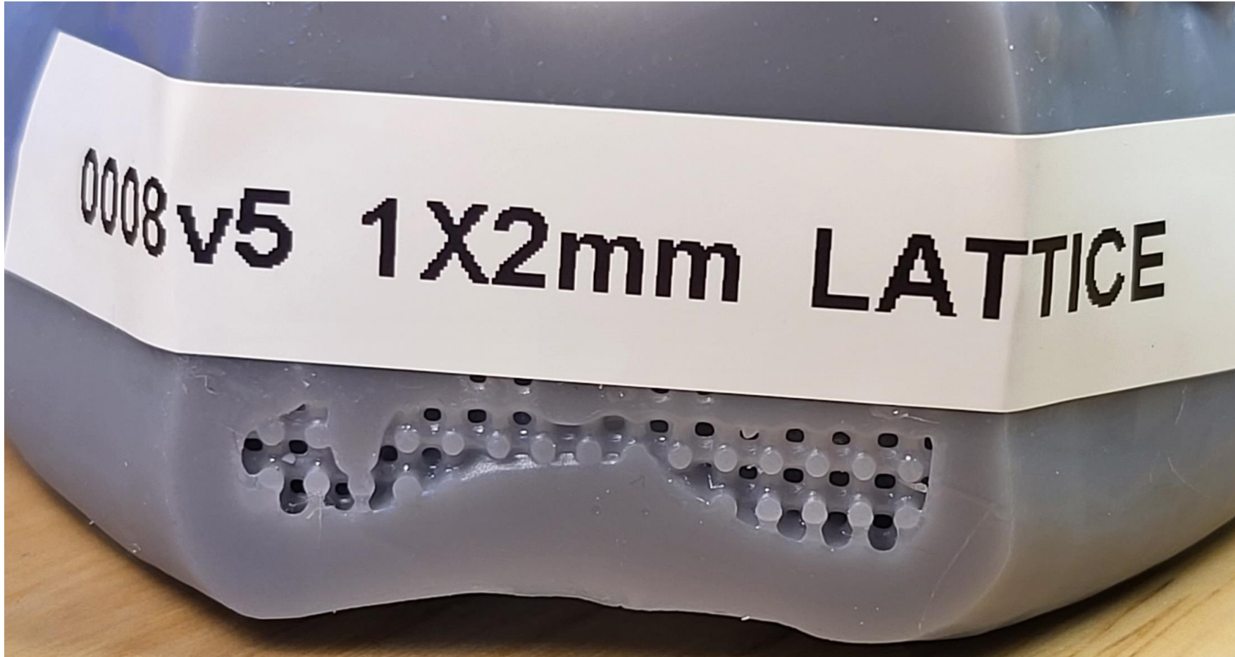
Error during print (Can see internal lattice)
