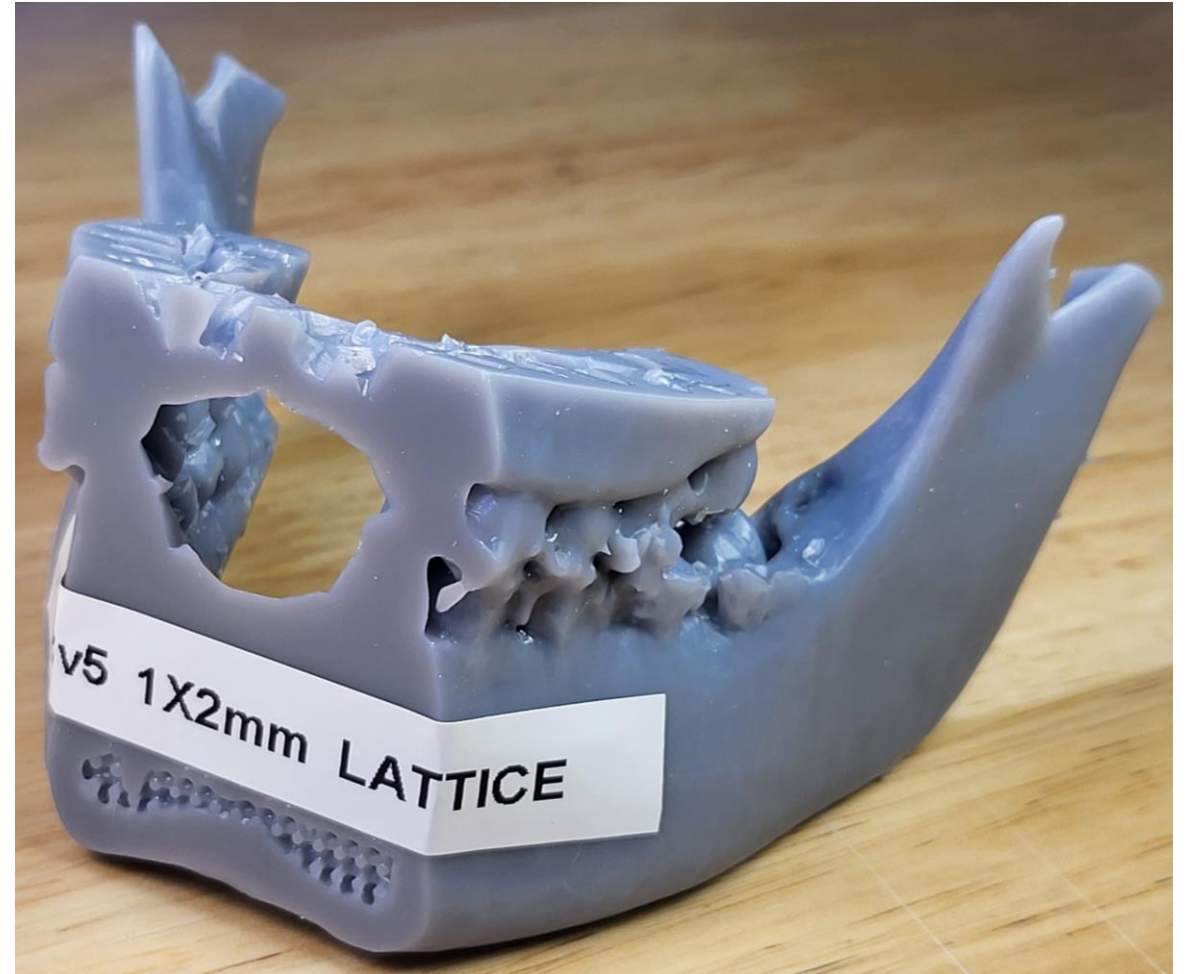
Error during print (Can see internal lattice)
