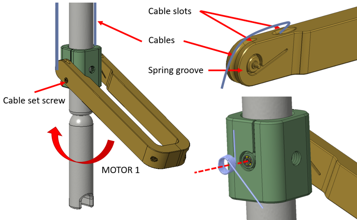
Figure 5. Swing mechanism of suture tensioning device showing the lever motion, cables, cable set screw, cable slots and spring grooves.
