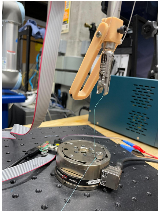
Figure 7 Force sensor setup below the STAR arm so that the thread is orthogonal to the table.
