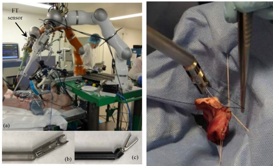
Figure 1a. (left) STAR autonomous 2-arm open environment setup [1]. 1b (right) STAR robot with manual suture tensioning management [2]
