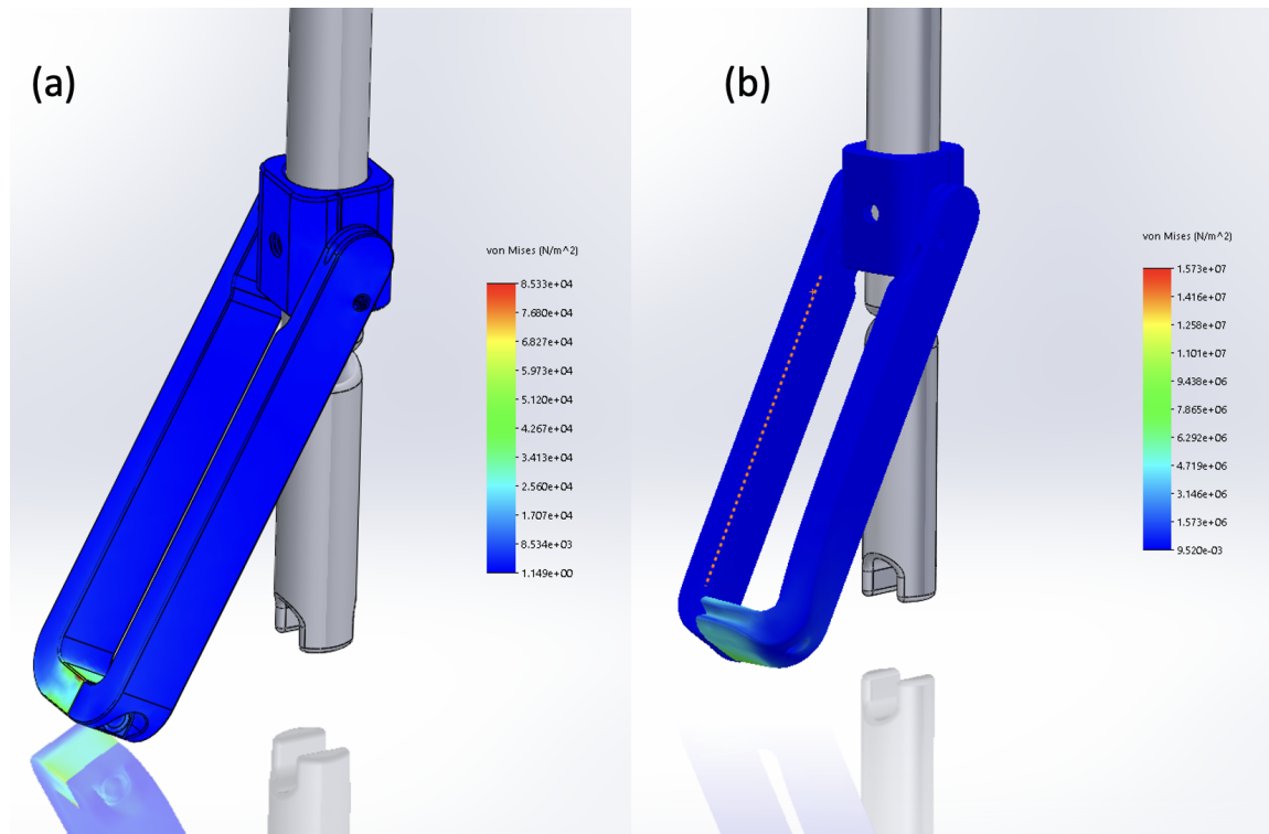
Figure 9: FEA results of the SMD: a) under normal tension force 0.6N b) under maximum tolerance with deformations.
