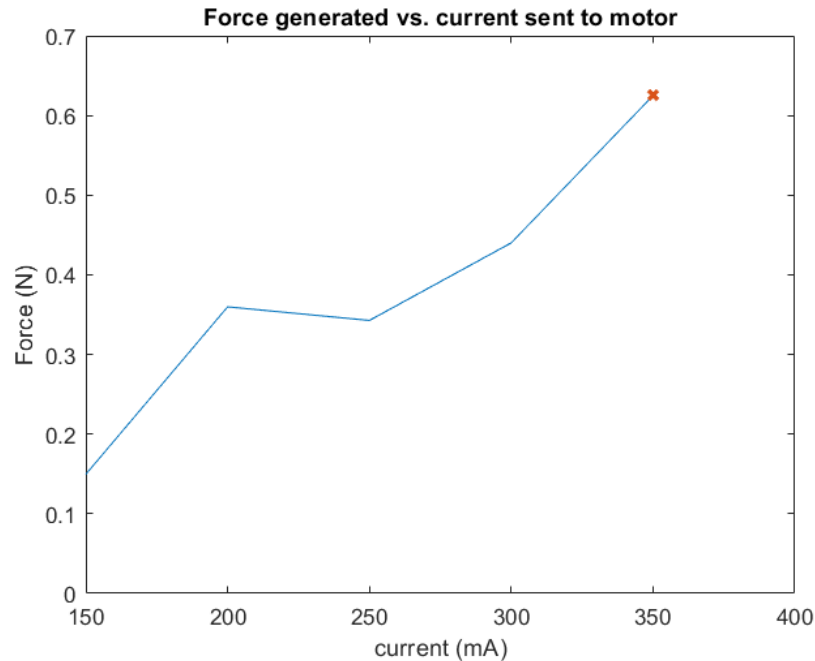
Figure 10 Force Testing Results. Red x indicates mechanical failure.
