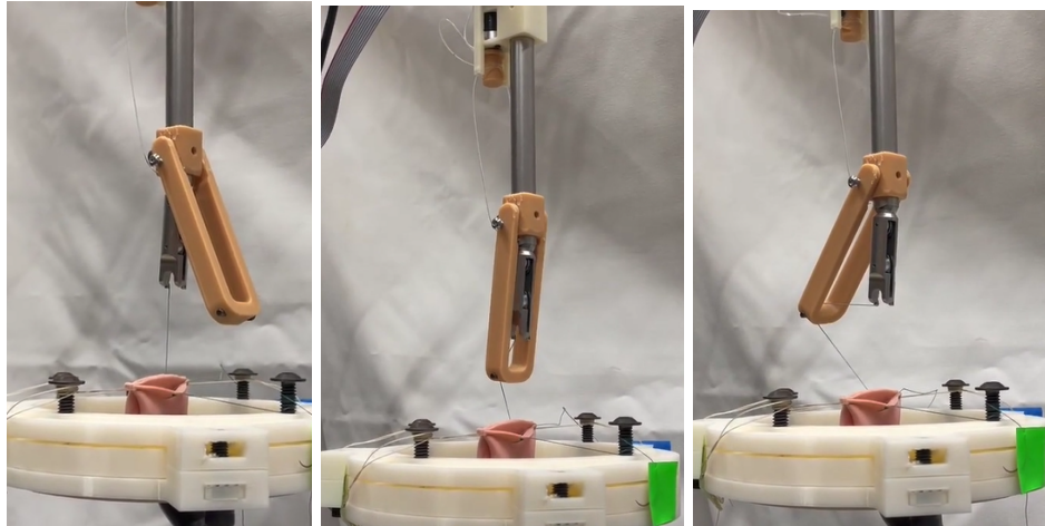
Figure 8. Synthetic Bowel Testing swing mechanism in starting position (left), contact position (middle), and fully tensioning thread (right)
