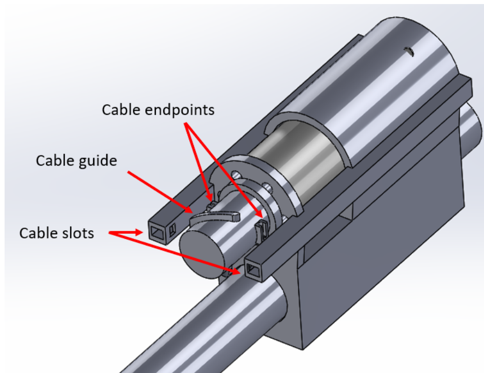
Figure 6. Transmission pointed on the Endo360 (grripper pointing down). The spool on the shaft of the motor shows the cable slots, guides and endpoints.
