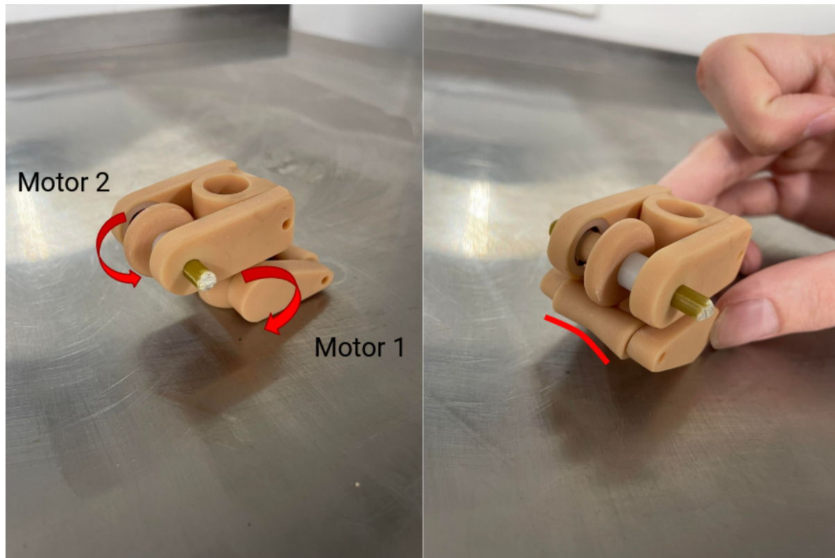
Figure 3. Roller mechanism of suture tensioning device showing the stationary, the swinging part and the fixed roller which tensions the suture. Note how the fixed and swinging roller have a complementary shape.
