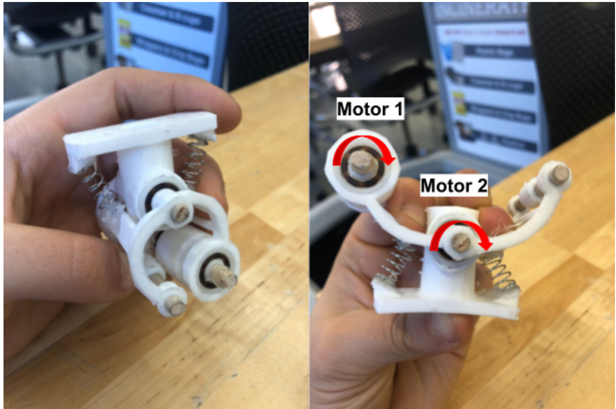
Figure 4a (left) Gripper design in closed position. 4b (right) gripper design in open position. The springs are responsible for the closing of the mechanism. Motor 1 tensions the thread.
