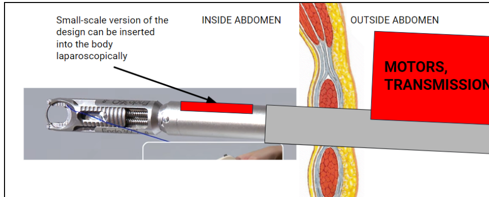
Figure 2: Diagram of project goal: small-scale mechanism which attaches to the STAR suturing end effector and can be inserted into the abdomen laparoscopically to autonomously manage suture tensioning.
