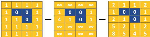
Fig. 7. Two-step transform in the 2D Euclidean Transform used to compute the SDF grid. Adapted from [14].
