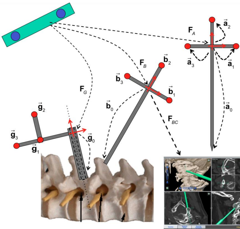
Fig. 4: Coordinate systems and positions associated with assignment
