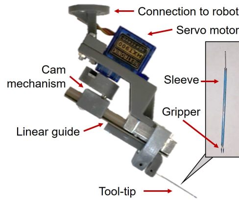
Fig. 3. Custom-designed micro-gripper used to grasp mosquitoes.
