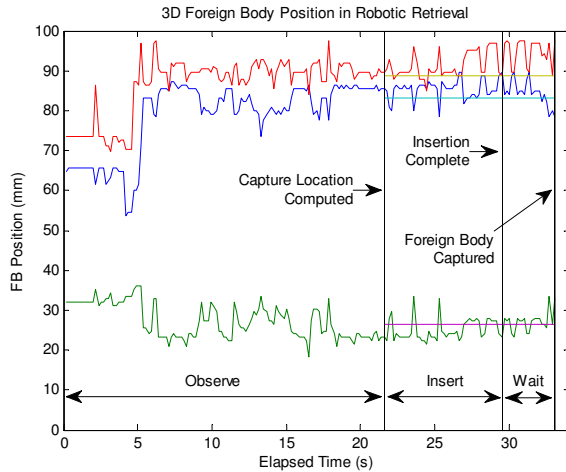
Fig. 6. Example three-axis foreign body motion trace during retrieval, with observation, insertion, and waiting phases annotated.
